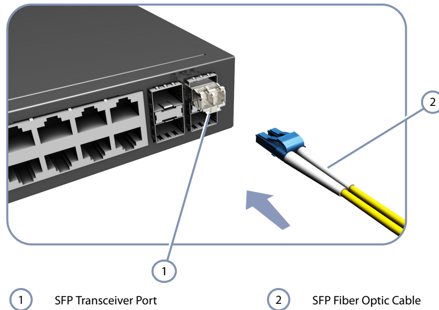
Figure 20: Making a Connection to an SFP Port
