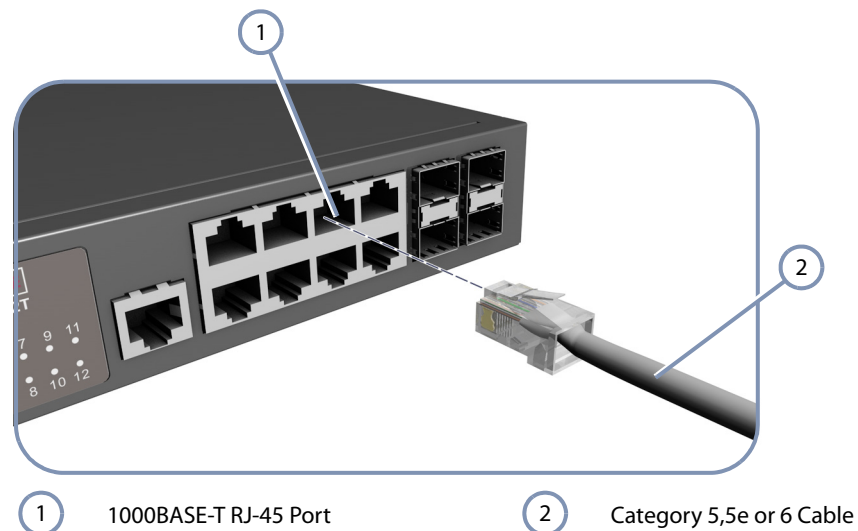
Figure 19: Making Twisted-Pair Connections
