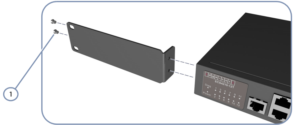
Figure 9: Attaching the Extension Brackets
