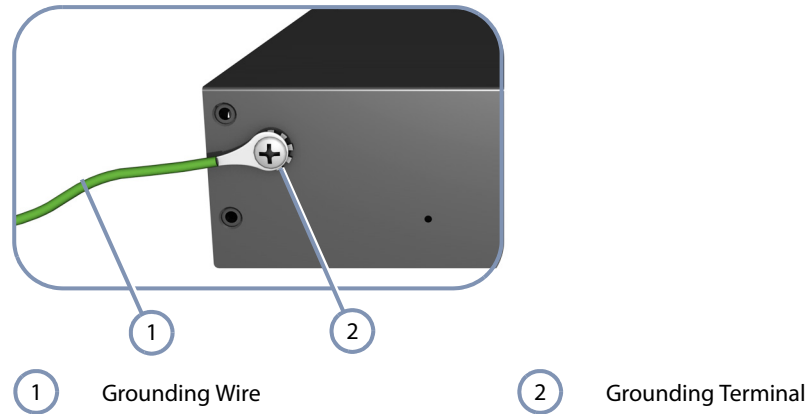
Figure 14: Grounding Terminal
