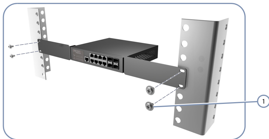
Figure 10: Installing the Switch in a Rack
