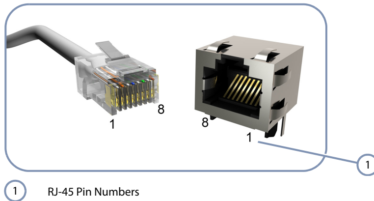
Figure 18: RJ-45 Connector
