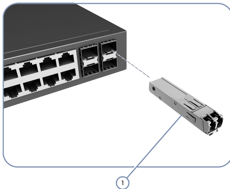
Figure 17: Inserting an SFP Transceiver into a Slot
