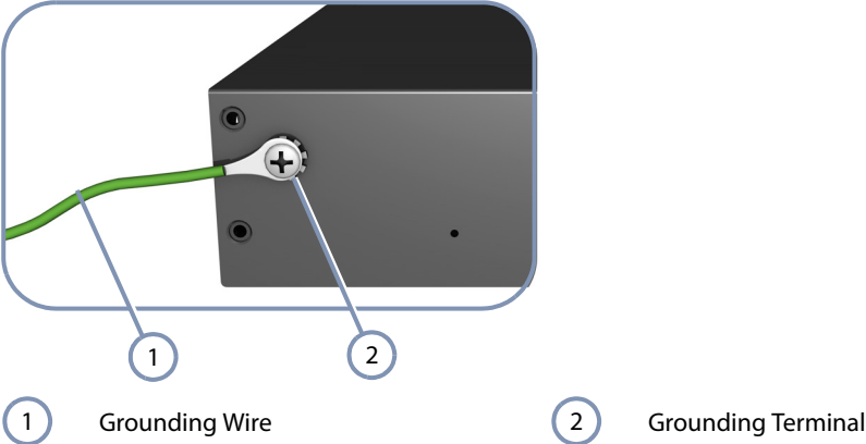
Figure 4: Grounding Terminal
